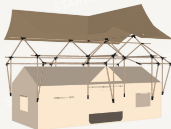
(3D Render-Assembly View)
