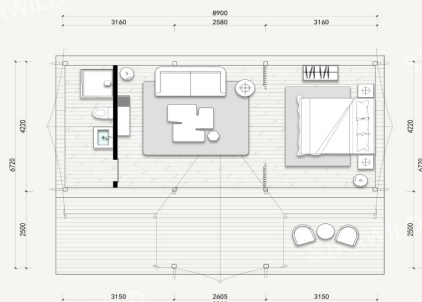
(Floor Plan)
