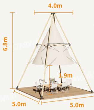
(3D Render-Assembly View)
