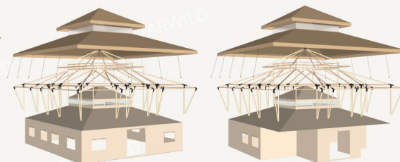
(3D Render-Exploded View)
