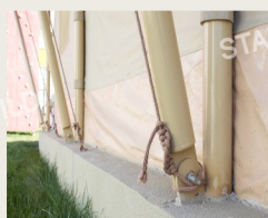
Ground Anchoring
