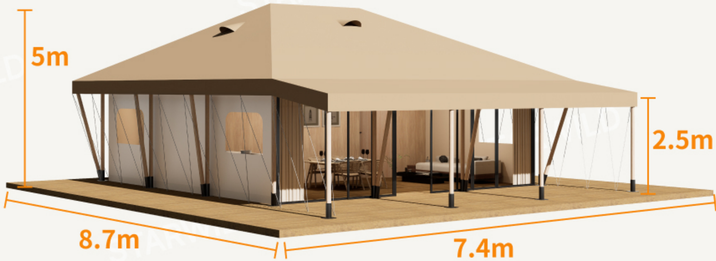
(3D Render-Assembly View)
