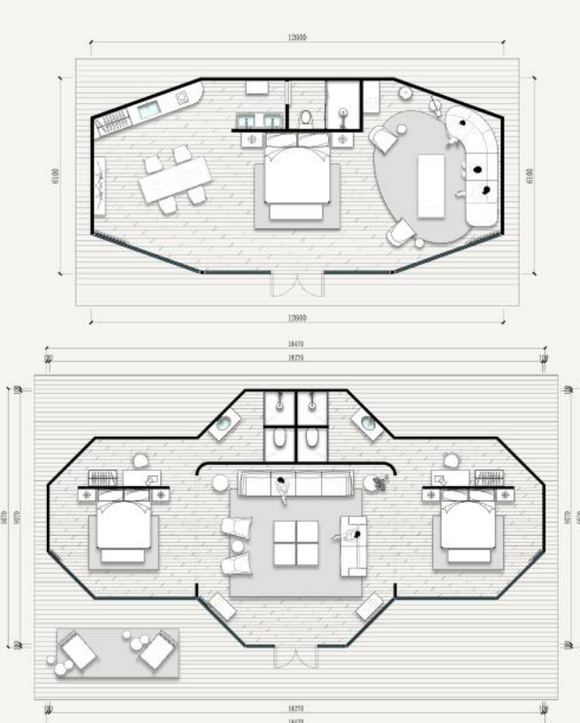
(Floor Plan)
